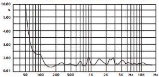
Distortion (THD< 5% 1W, 1m, 100Hz-10kHz)
