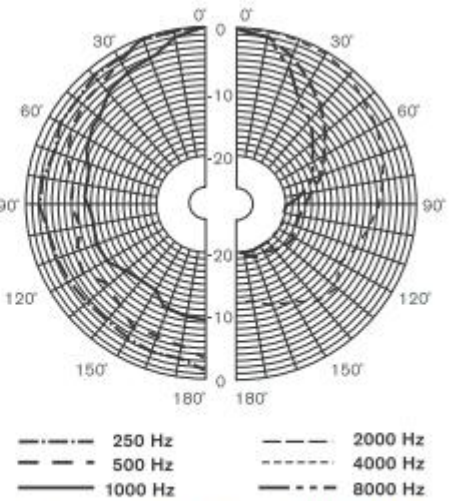
Horizontal directivity pattern
