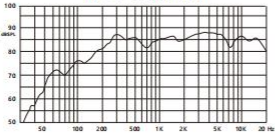
Frequency Response (dB SPL, 1W, 1m)
